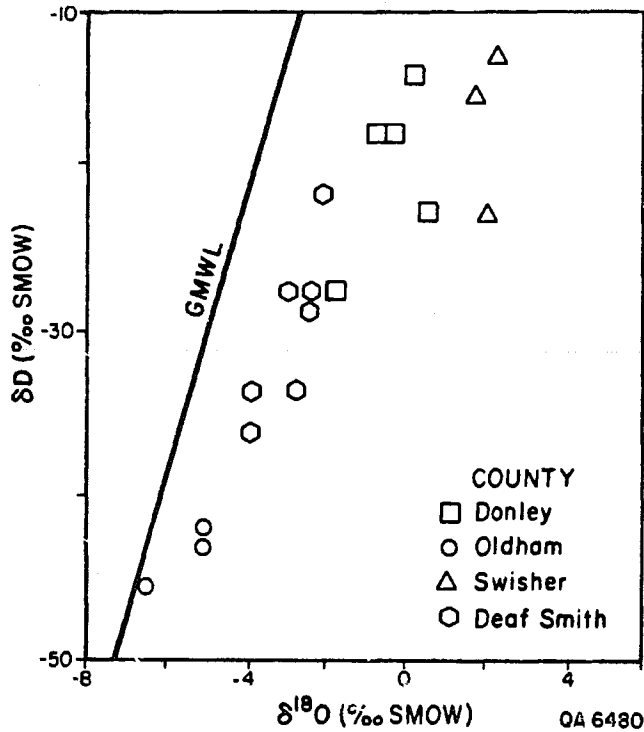
Fig. 7. Hydrogen and oxygen isotopic composition of waters from the deep-brine aquifers in the Palo Duro Basin. Waters from Oldham and Deaf Smith Counties in the western part of the basin trend toward the isotopic composition for meteoric water in the region. These waters are not isotopically equilibrated for their depth (temperature) of sampling. In contrast, waters from Donley and Swisher Counties (the eastern part of the basin) are in isotopic equilibrium for their depth of sampling (from Fisher and Kreitler, 1987). GMWL is Global Meteoric Water Line (Craig, 1961).
