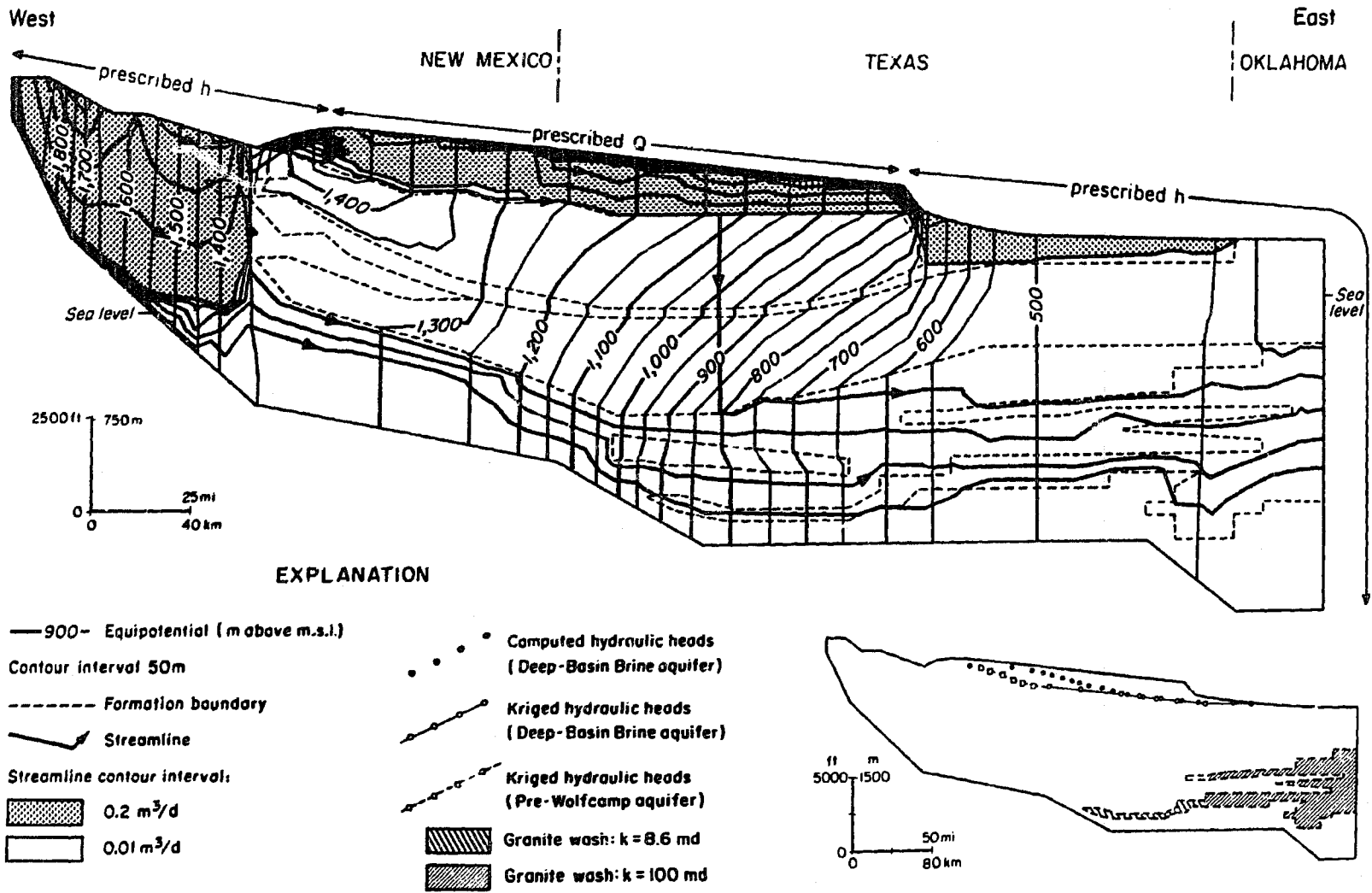
Fig. 3. Schematic west-east hydrogeologic section of the Palo Duro Basin with simulated potentiometric contours and streamlines (from Senger et al., 1987).
